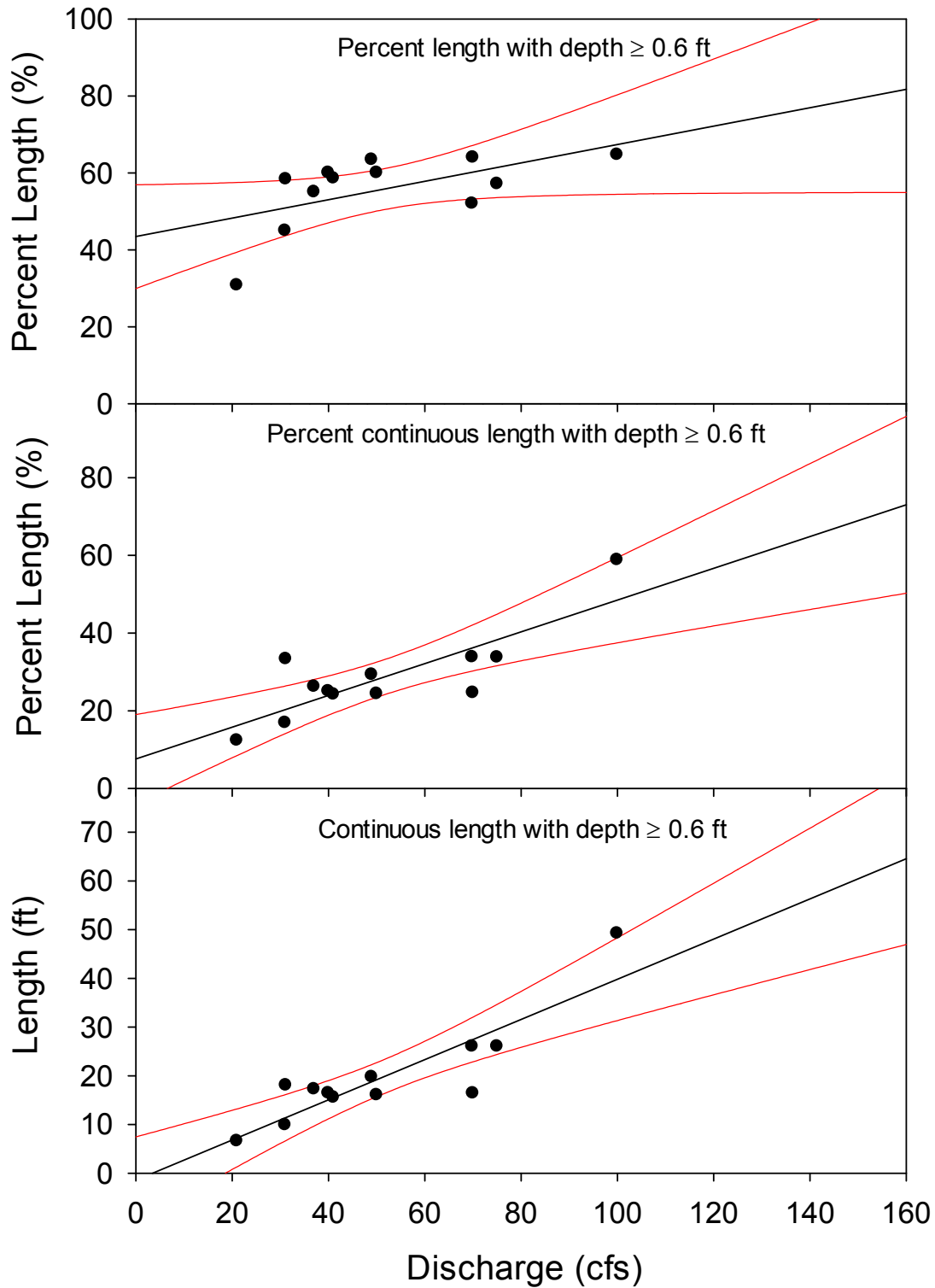
Appendix 12. Linear regression (and 95% CI) between Robles discharge and water depth at Site 8 downstream of Robles Fish Facility.
