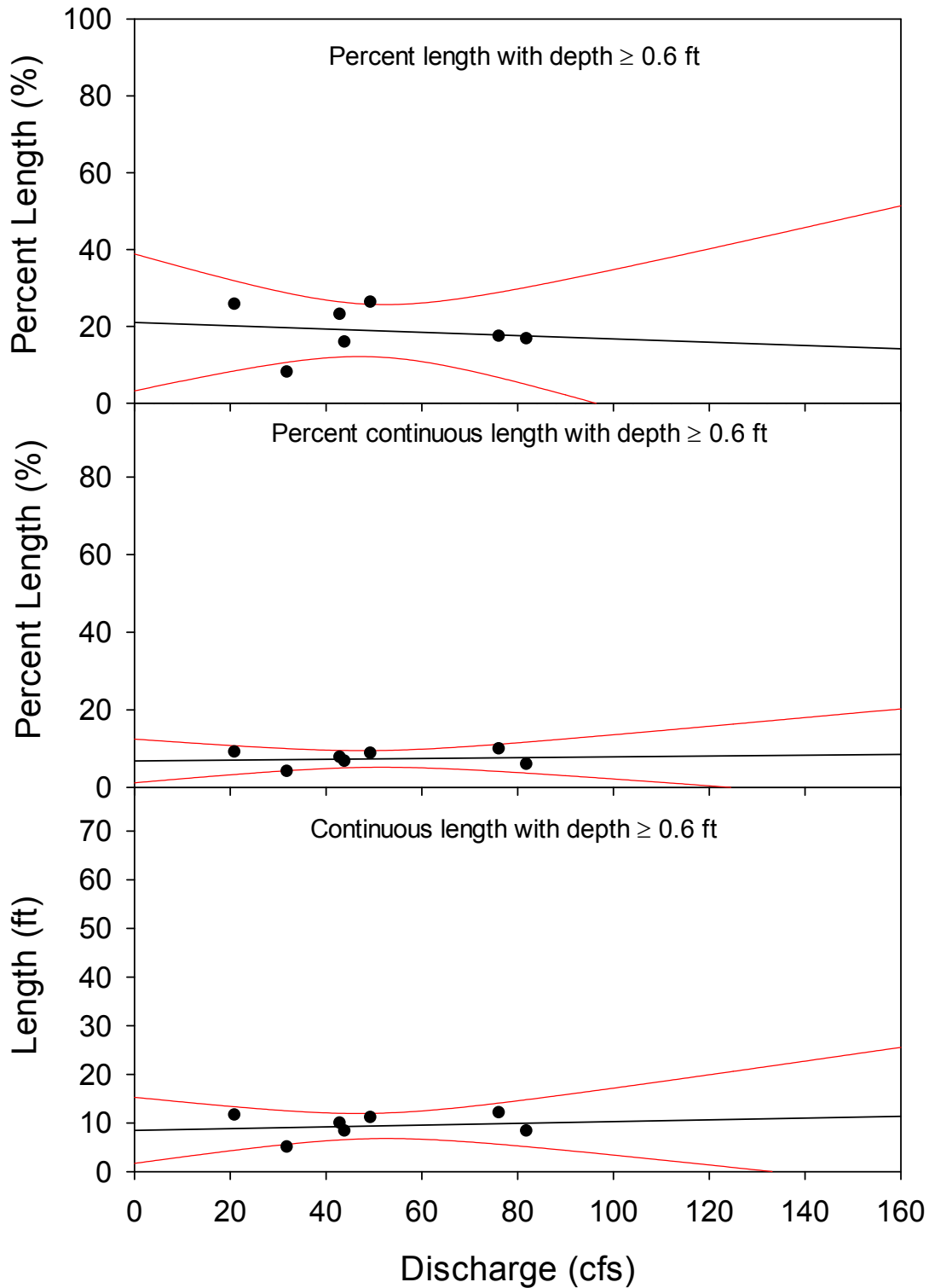
Appendix 5. Linear regression (and 95% CI) between Robles discharge and water depth at Site 3-1 near Casitas Springs.
