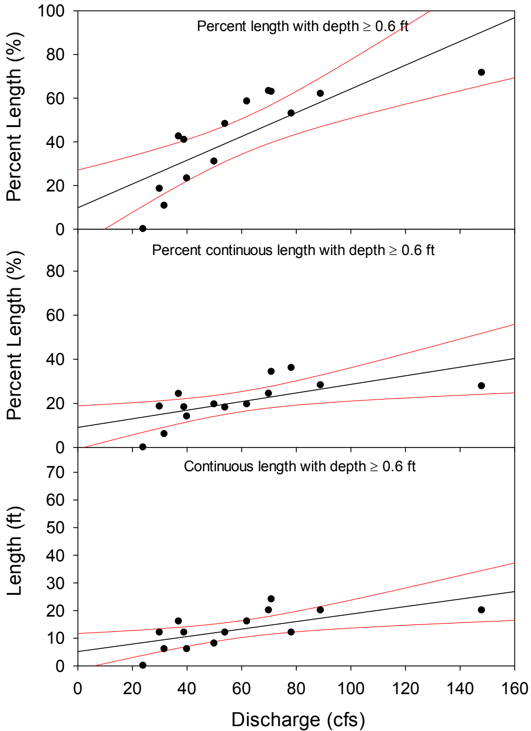
Appendix 13. Linear regression (and 95% CI) between Robles discharge and water depth at Site 9 upstream of Hwy 150 bridge.
