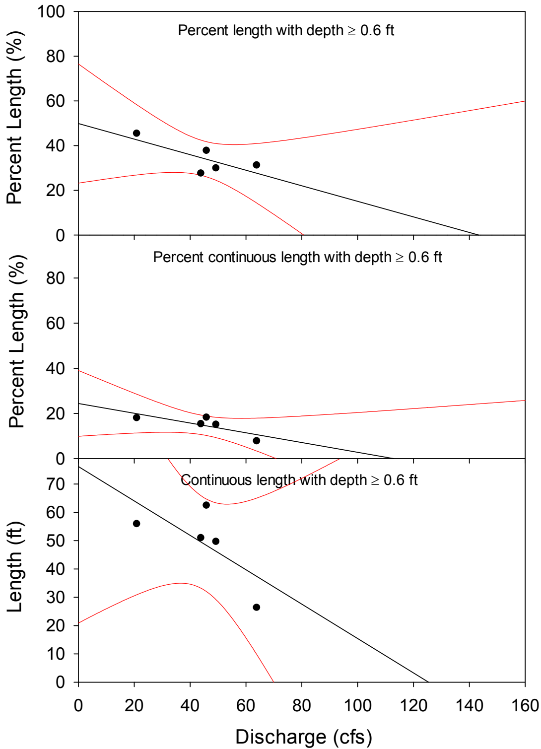
Appendix 4. Linear regression (and 95% CI) between Robles discharge and water depth at Site 2 near Ojai Valley Sanitation District treatment plant.
