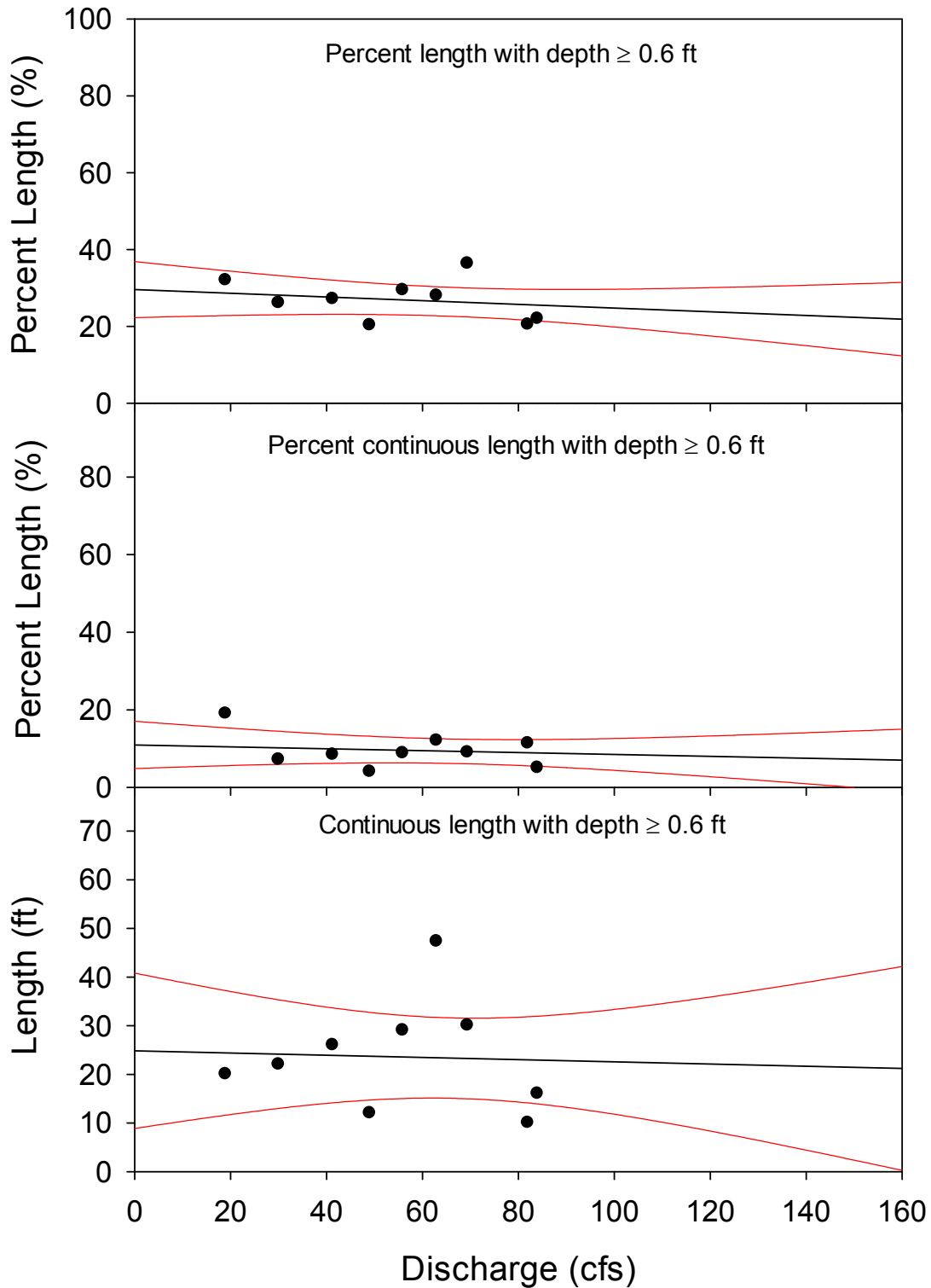
Appendix 6. Linear regression (and 95% CI) between Robles discharge and water depth at Site 3-2 near Casitas Springs.
