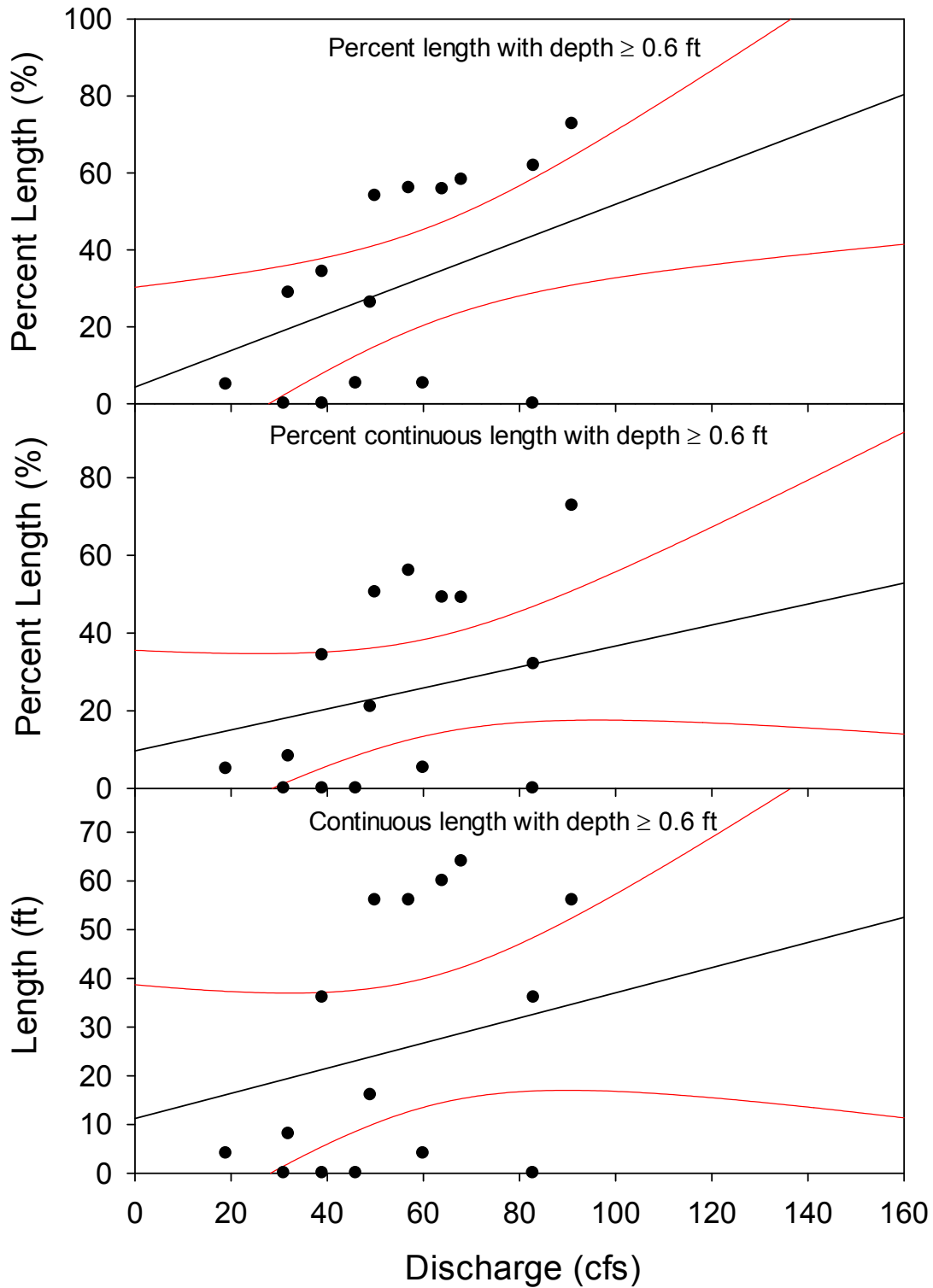
Appendix 14. Linear regression (and 95% CI) between Robles discharge and water depth at Site 10 downstream of Casitas Springs.
