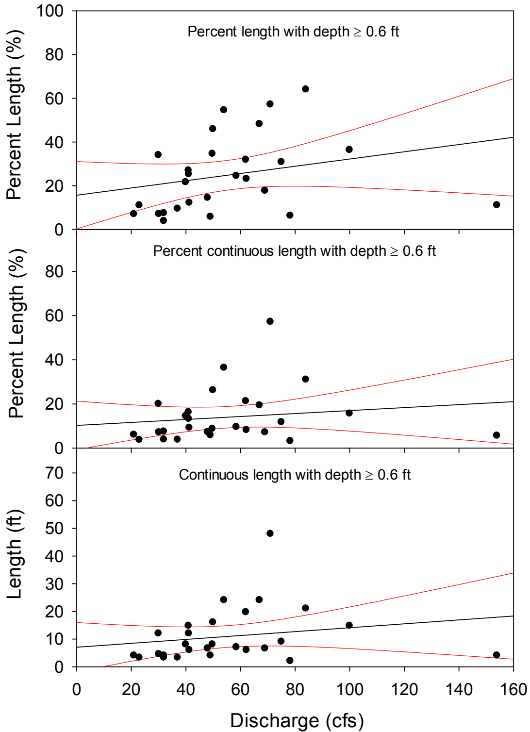
Appendix 10. Linear regression (and 95% CI) between Robles discharge and water depth at Site 6 upstream of Santa Ana bridge.
