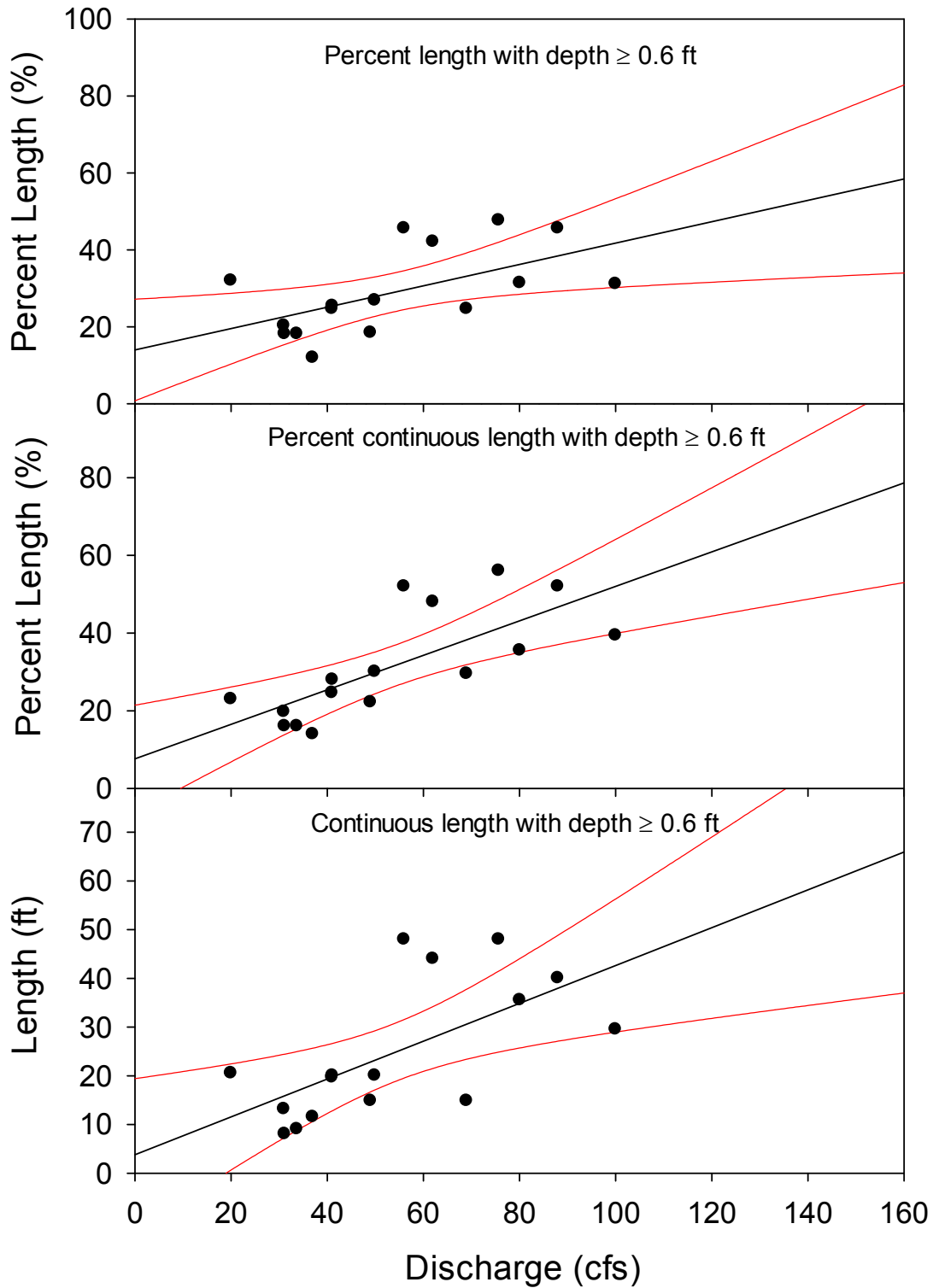
Appendix 11. Linear regression (and 95% CI) between Robles discharge and water depth at Site 7 upstream of Hwy 150 bridge.
