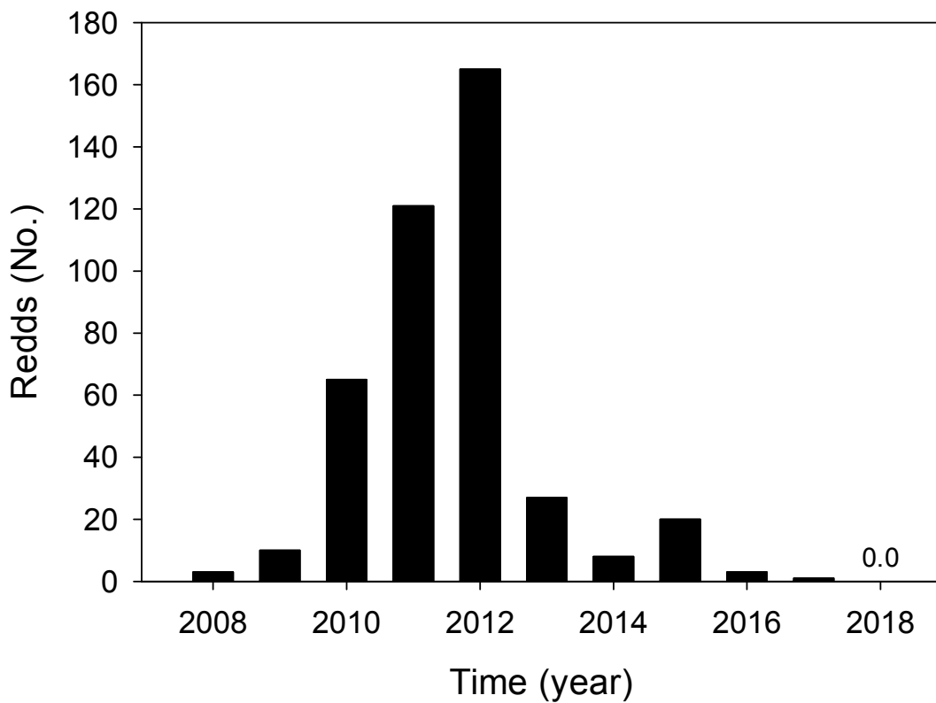
Appendix 28. Total number of O. mykiss redds counted at index spawning sites from 2008 through 2018 spawning years.
