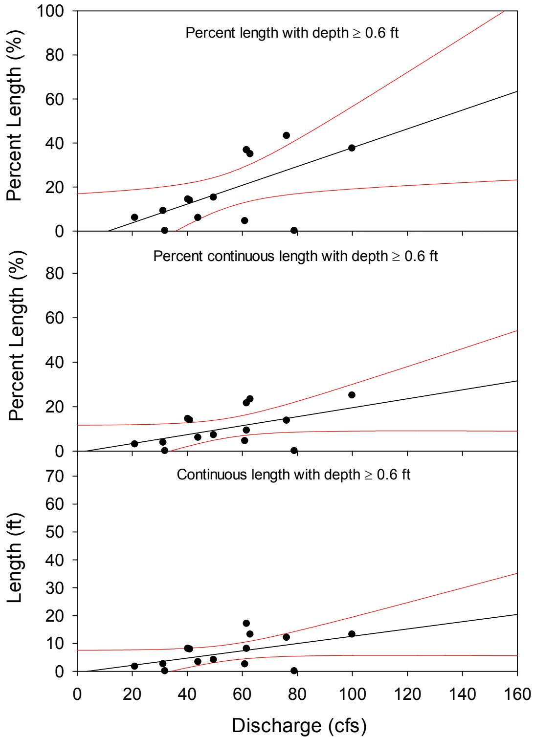
Appendix 7. Linear regression (and 95% CI) between Robles discharge and water depth at Site 4 upstream of San Antonio Creek confluence.
