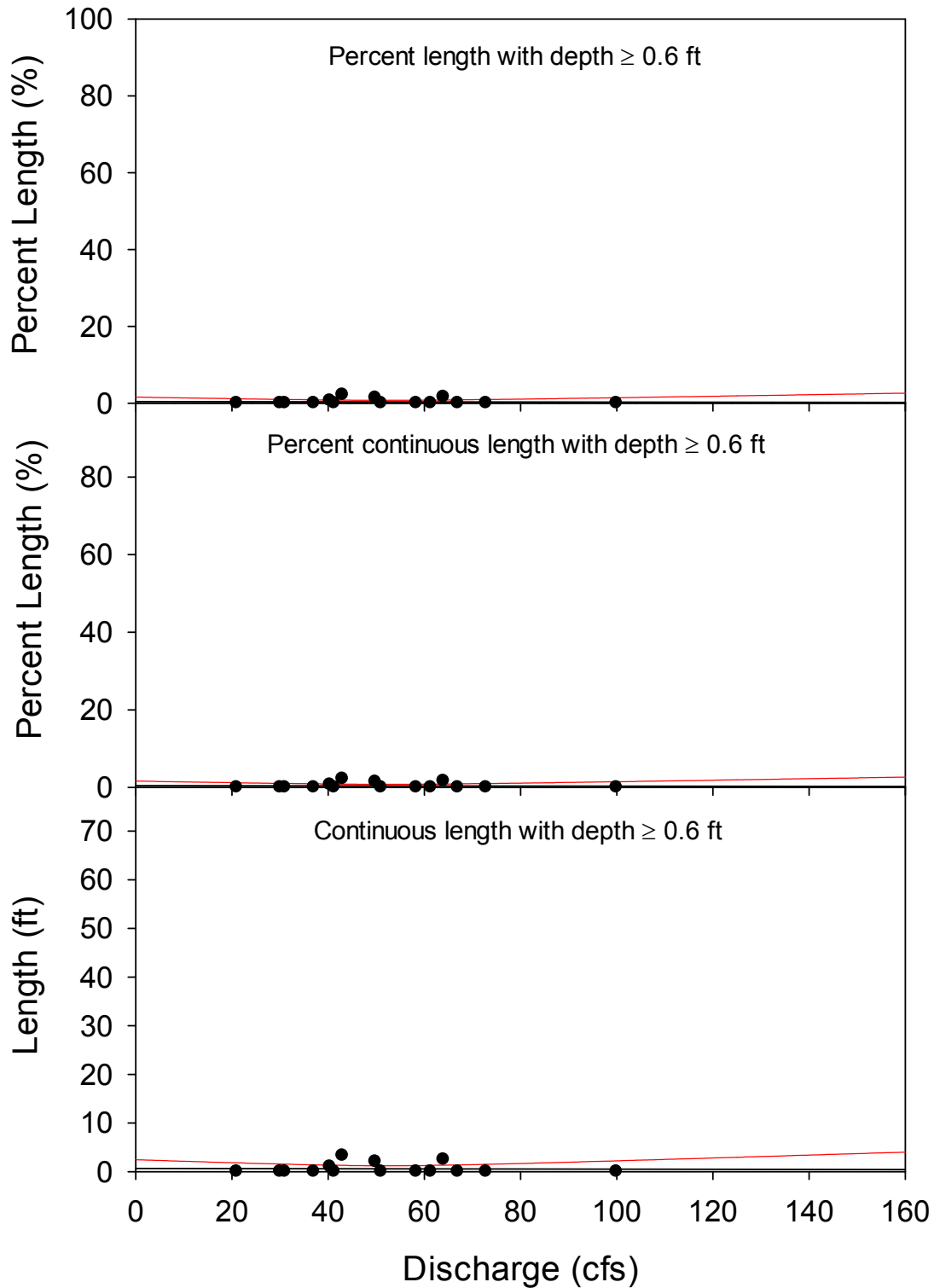
Appendix 8. Linear regression (and 95% CI) between Robles discharge and water depth at Site 5-1 downstream of Santa Ana Bridge.
