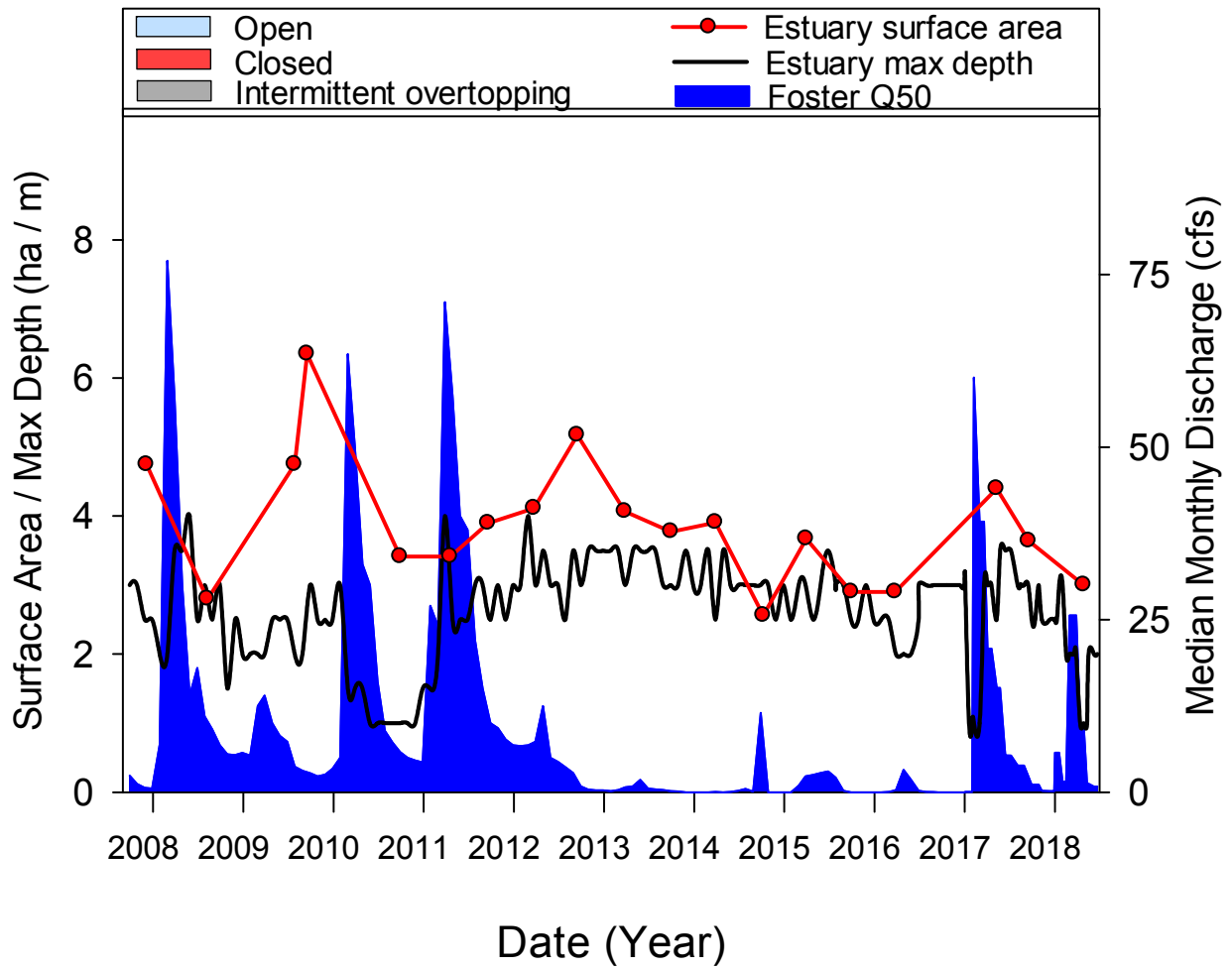
Appendix 31. Ventura River estuary/lagoon water depth, surface area, sandbar status, and discharge at Foster Park from 2008 to 2018.
