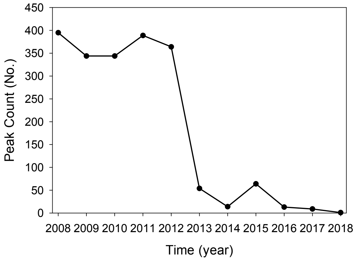
Appendix 25. Peak snorkel counts of O. mykiss during the period 2008-2018 at survey index sites in the Ventura Basin.
