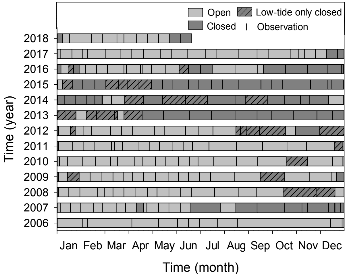
Appendix 17. Sandbar status at the mouth of the Ventura River from 2006 through July of 2018. Each observation is indicated by vertical lines and the sandbar status was assumed to remain unchanged until the next observation.
