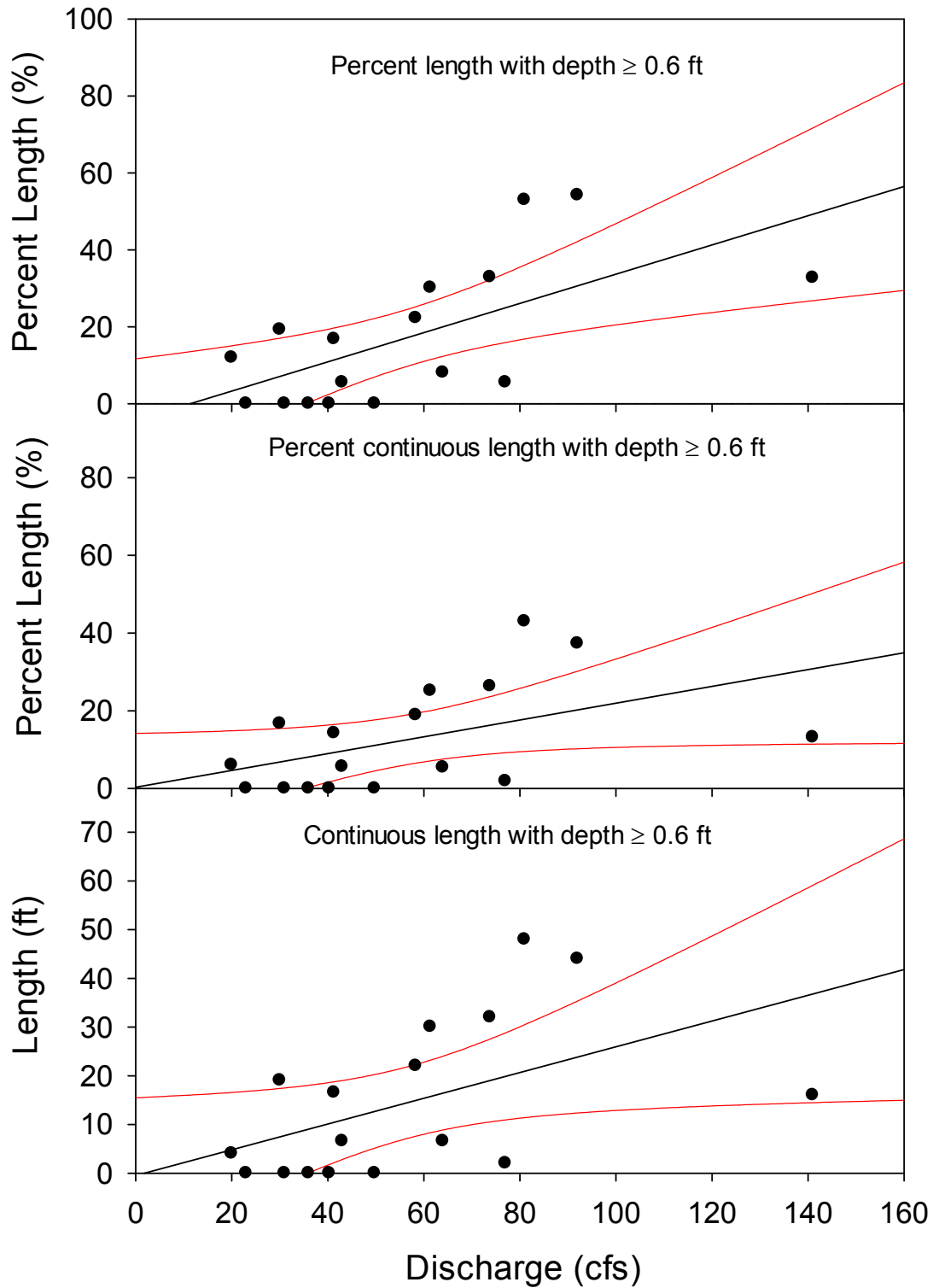
Appendix 9. Linear regression (and 95% CI) between Robles discharge and water depth at Site 5-2 downstream of Santa Ana Bridge.
